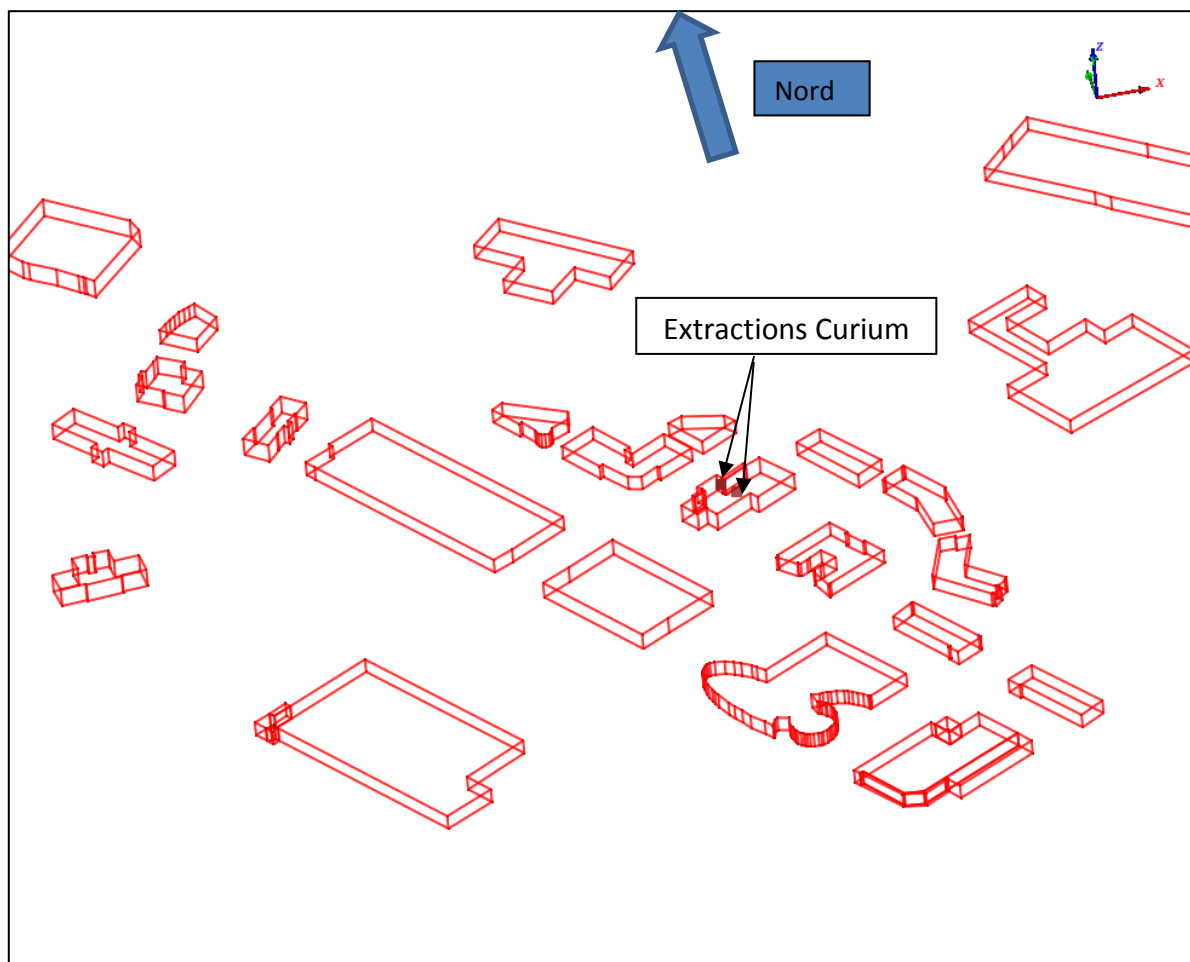
Figure 4: Maquette 3D de simulation
